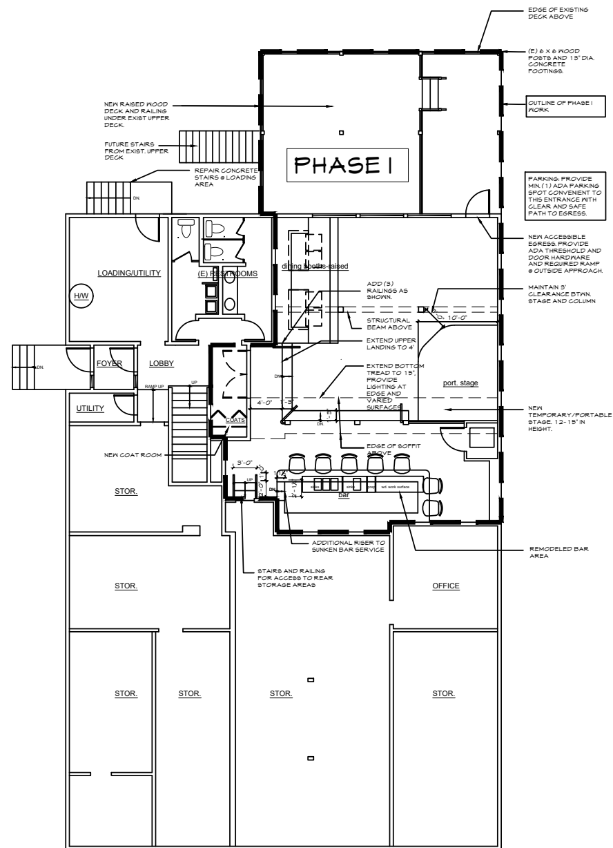
LOWER LEVEL EXIST. AND PROPOSED T BAR REMODEL-INCLUDES PROJECT PHASES
